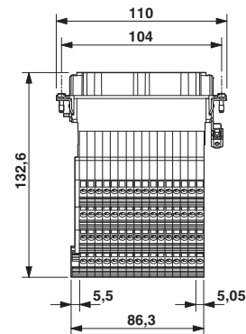
Dimensional drawing
